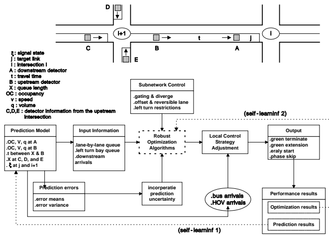
Figure 4. Block diagram of fuzzy neural traffic light
