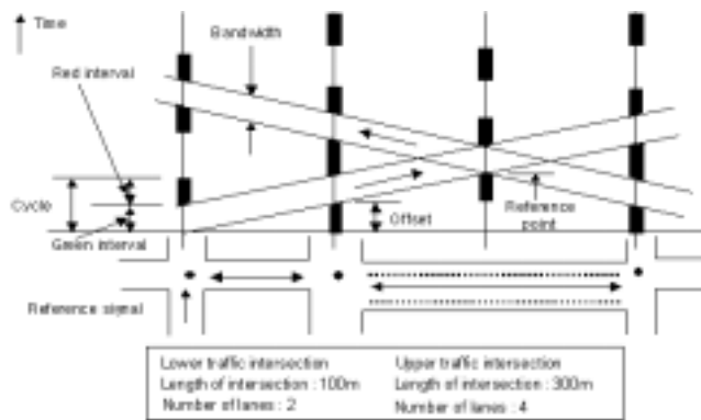
Figure 3. Optimal green time depending on lower and upper traffic intersection
