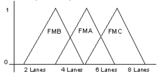
Figure 7. Adaptive fuzzy control depending on number of lane
